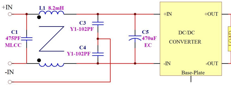
Measured conductive level of COE48050abcd-XXXXX and referenced filter circuit
